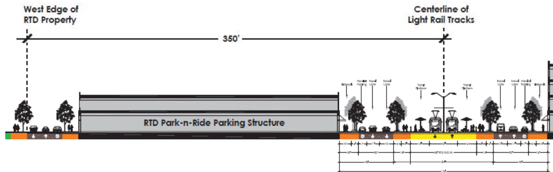
Figure 30. Proposed RTD Property Cross-Section
