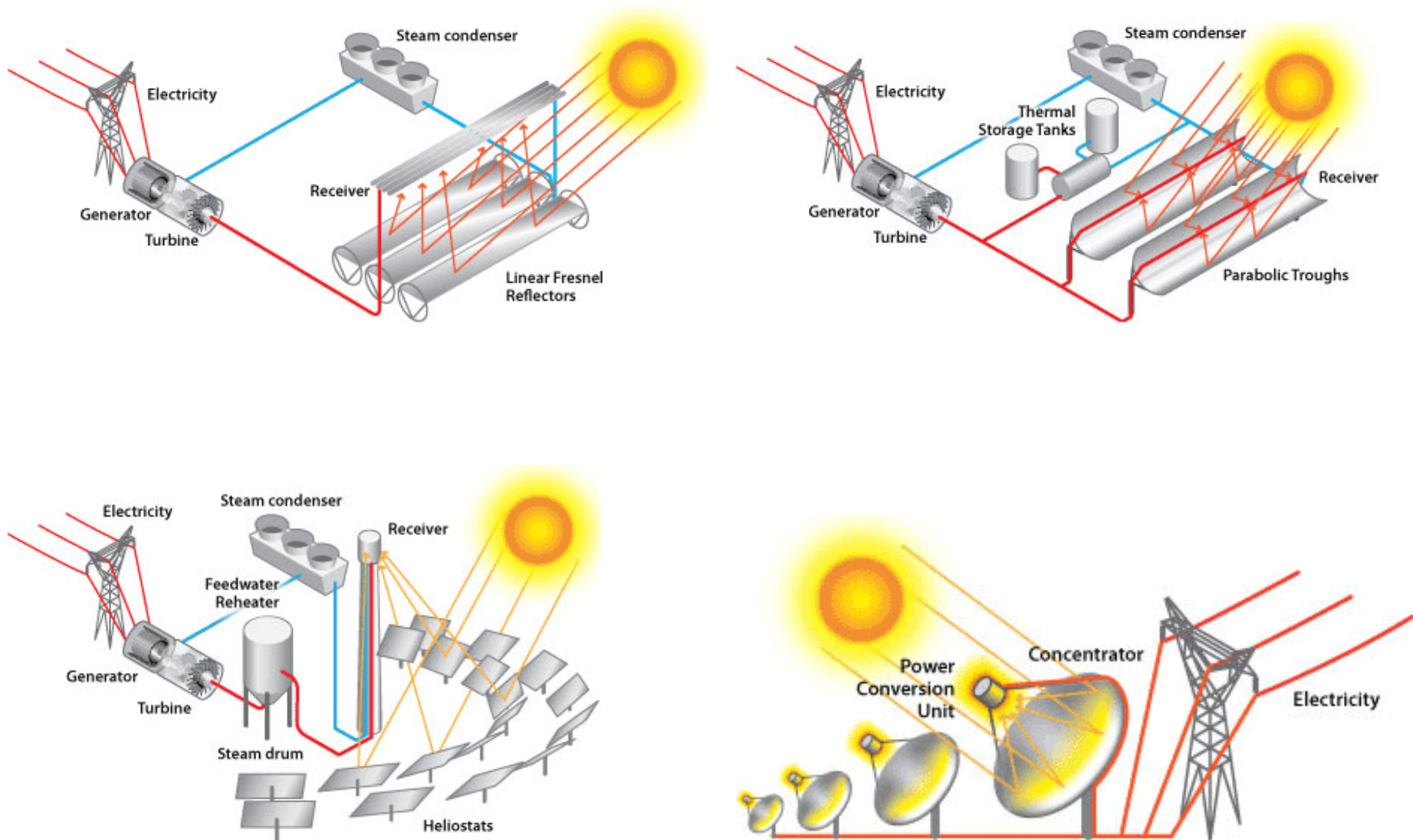
Figure 8.8: The four primary CSP technologies
